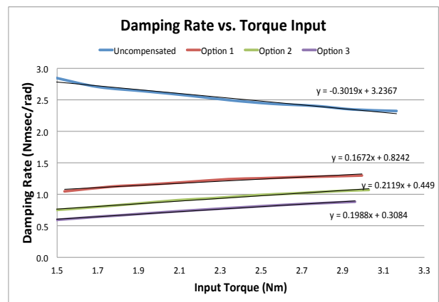
Figure 5 - Damping Rate vs. Torque Input
