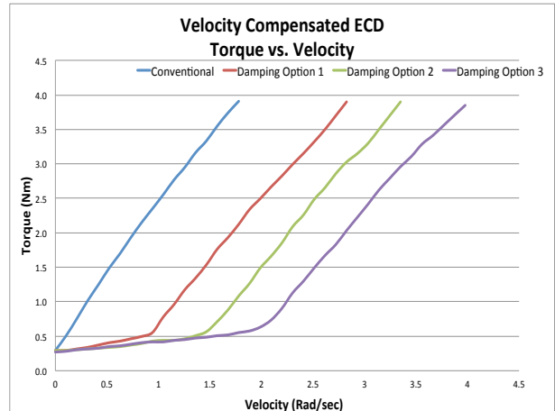
Figure 2 - Compensated Velocity Damper Options
